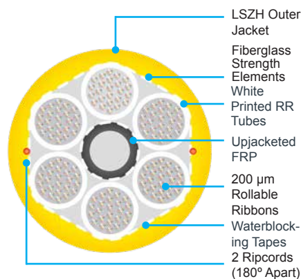
AccuTube 200 µm Rollable Ribbon Outdoor/Indoor Building Cable Cross-section
