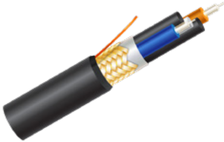
2-Fiber Heavy-Duty Breakout
