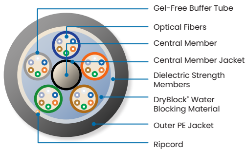
PowerGuide ShortSpan DT Cable Cross-Section
